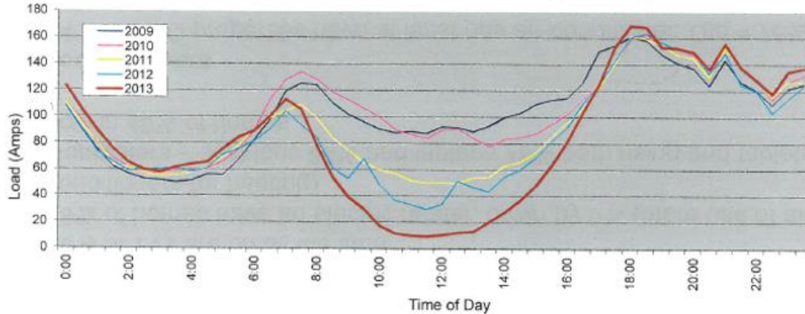
Typical SEQ 11,000 volt powerline with high solar penetration
