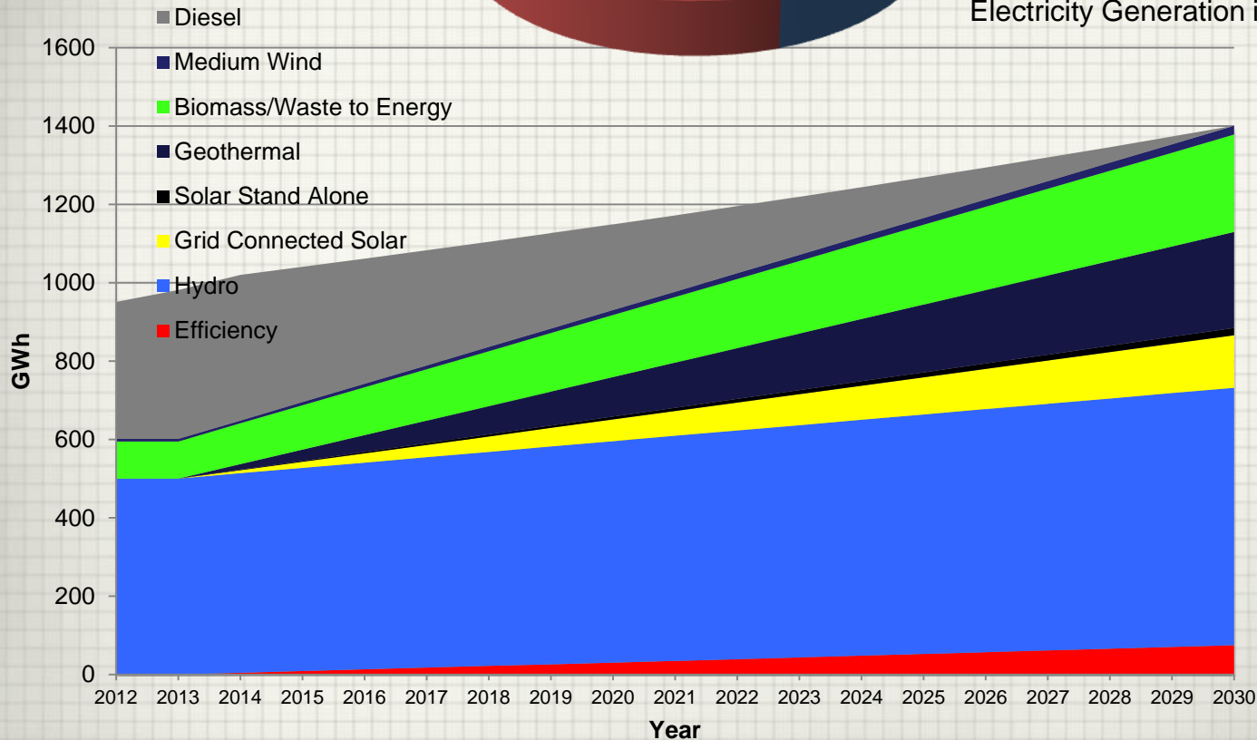
Electricity Generation in Fiji by Source (FEA-2014 Data)
