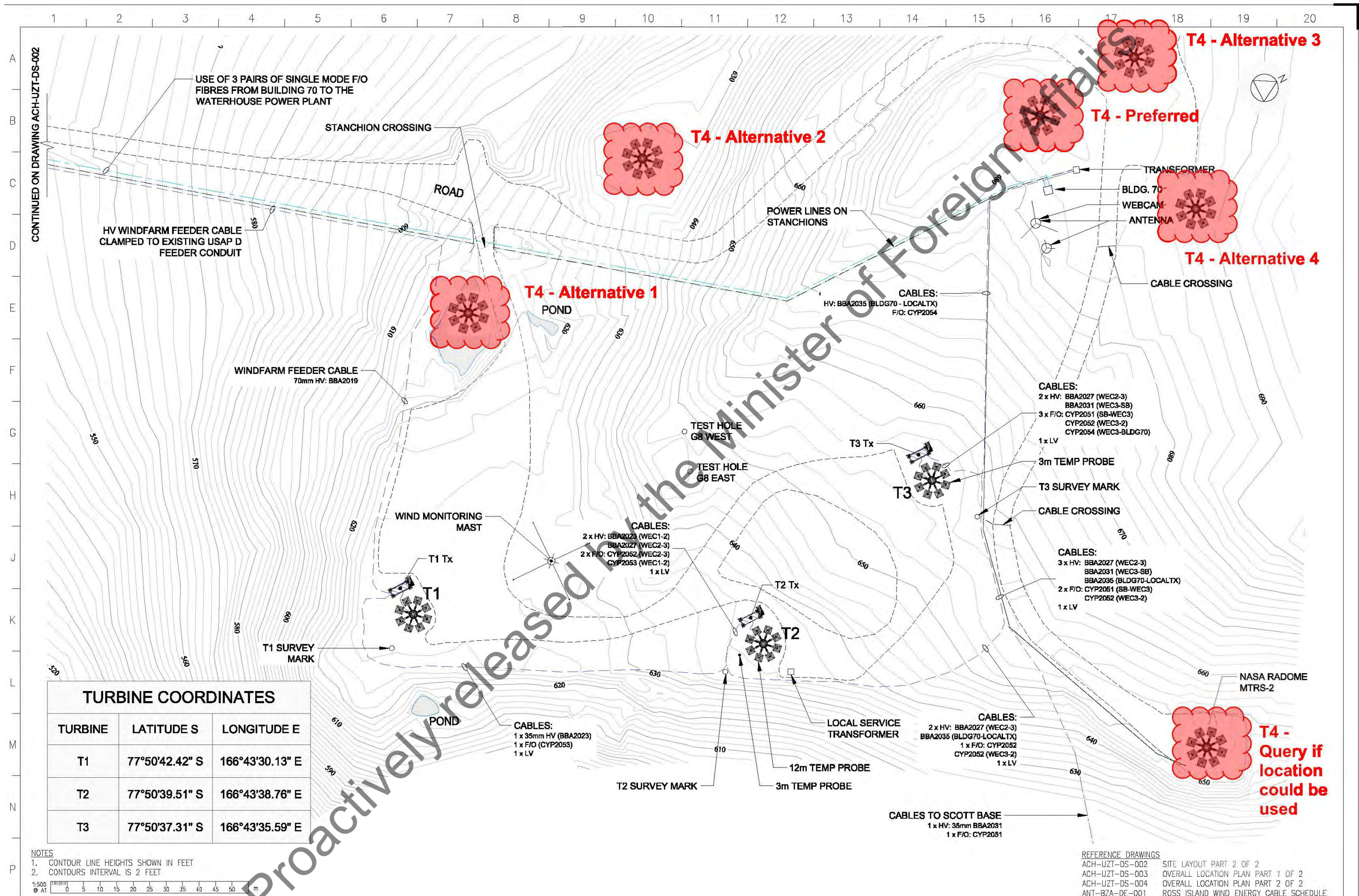
Figure 55: Current RIWE turbine locations (T1, T2 and T3) with alternative option for a fourth location (T4).
