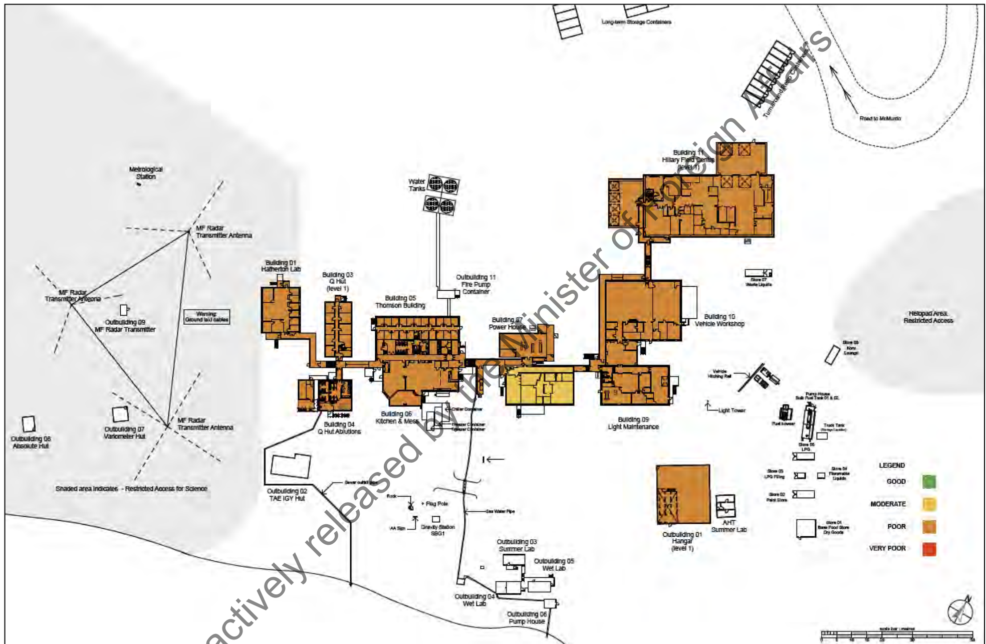
Figure 10: Existing Scott Base site plan with building condition rating.
